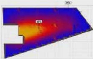
DYNAMIC DAYLIGHT AUTONOMY SIMULATION FOR A BASE BUILDING WITH TYPICAL CURTAIN WALL DURING WINTER
